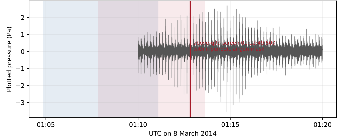
H08S Figure 9e: conditional reception windows and screened periodic feature
