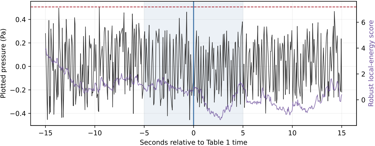
H08S Figure 9d: conditional reception windows and screened periodic feature
