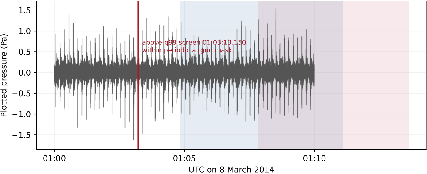
H08S Figure 9d: conditional reception windows and screened periodic feature
