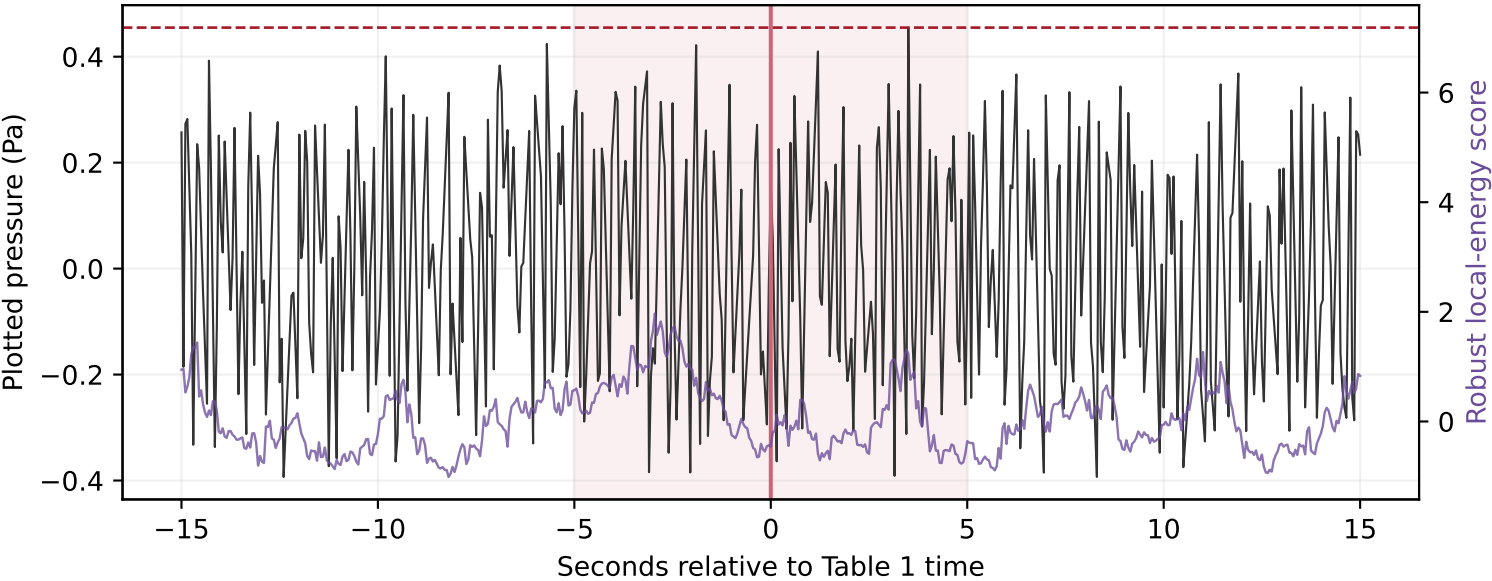
H08S Figure 9e: conditional reception windows and screened periodic feature
